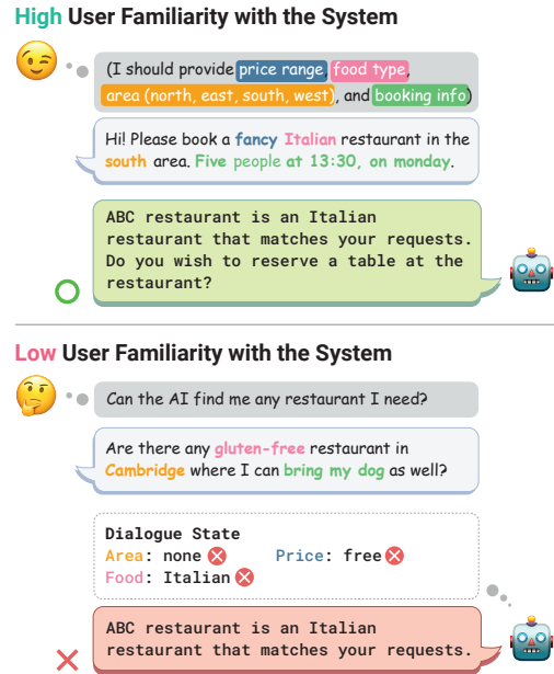
Figure 1: Contrastive dialogues according to user familiarity with the system. Users with high familiarity converse with the system within the predefined scenario since they already know the system well. However, users with low familiarity are more likely to talk about a broad range of topics beyond the system’s capacities leading to the erroneous response of the system.
